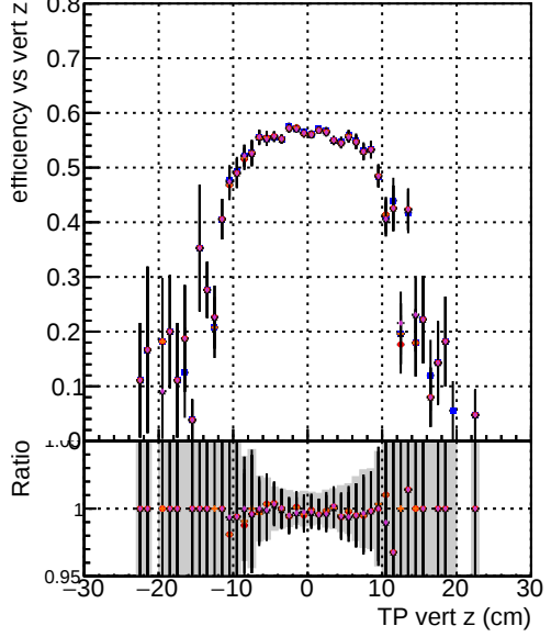
Efficiency vs. TP vert z — DOM mkFit TToriginal — DOM mkFit TTNEWHSMSS95 — DOM mkFit TTNEWHSMSS95ch2 — DOM mkFit TTNEWHSMSS95dpdg — DOM mkFit TTNEWHSMSS95dpdg ALLITERS-106
