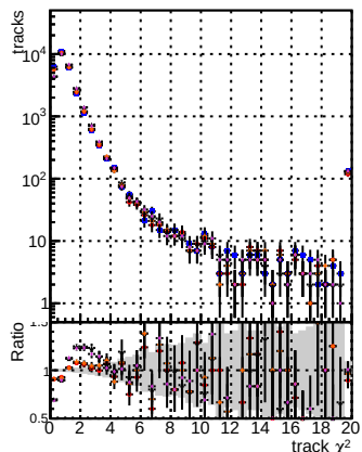
N of reco track vs. \chi^2 for BOM, mFit, TIT, Original vs, ALL ITERS-106, NEWISM3500, and ALL ITERS-106
