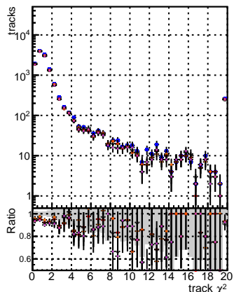
N of reco track vs. \chi^2 for various models: BSM mFit, Original vs. BSM mFit, NEWHSN39, ALL FTS-106, ALL FTS-106
