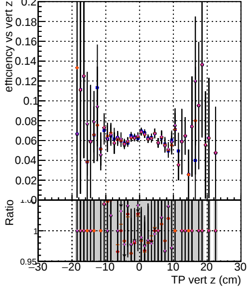
Efficiency vs. TP vert z DOM mkFit original DOM mkFit original-106 DOM mkFit TTNEWHSMS95 DOM mkFit TTNEWHSMS95chi2 DOM mkFit TTNEWHSMS95dpdg ALLITERS-106
