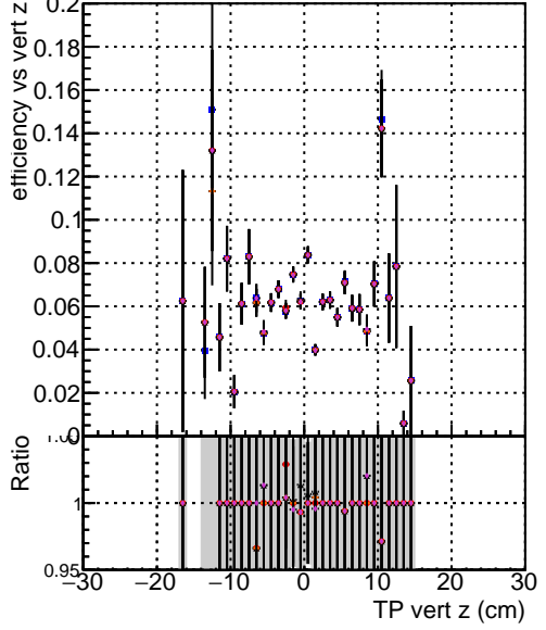
Efficiency vs vert z —●— DQM mkFit original_106 —●— DQM mkFit NEWHSM95 ALLITERS-106 —●— DQM mkFit NEWHSM95ch2 ALLITERS-106 —●— DQM mkFit NEWHSM95dpdg ALLITERS-106
