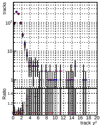
DOM mktFit TToriginal 106 ALLITERS-106 N of reco track vs. s NEWHSM93dpuz ALLITERS-106
