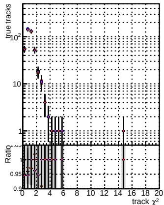
DOM mktFit TToriginal 106 ALLITERS-106 N of reco track vs. s NEWHSM93dpuz ALLITERS-106
