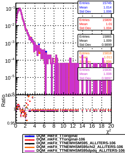
normalized \chi^2
