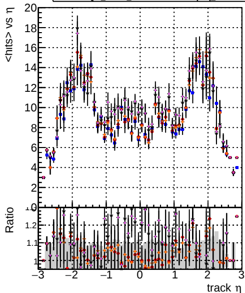
mean hit DOM mkFit TToriginal-106 DOM mkFit TTNEWHSMS95 ALLITERS-106 DOM mkFit TTNEWHSMS95ch2 ALLITERS-106 DOM mkFit TTNEWHSMS95dpdg ALLITERS-106
