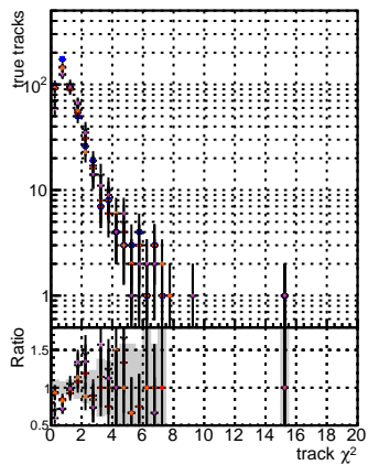
N of reco track vs. \chi^2 for different track types: DOM (black), mFit (red), T (blue), Original (green), New (orange). ALL LITERS 106, NEW LITERS 39, DOM LITERS 39, mFit LITERS 39, T LITERS 39, Original LITERS 39, New LITERS 39.
