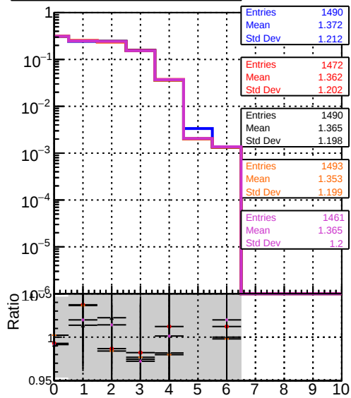
mean hit DOM mkFit Toriginal-106 DOM mkFit TNEWHSMS95 ALLITERS-106 DOM mkFit TNEWHSMS95chi2 ALLITERS-106 DOM mkFit TNEWHSMS95dpdg ALLITERS-106
