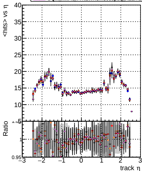
mean hit DOM mkFit Toriginal-106 DOM mkFit TNEWHSMS95 ALLITERS-106 DOM mkFit TNEWHSMS95chi2 ALLITERS-106 DOM mkFit TNEWHSMS95dpdg ALLITERS-106
