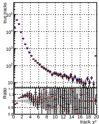
N of reco track vs. \chi^2 for BOM, mFit, TTFinal, and TTFinal vs. ALL LIPS-106
