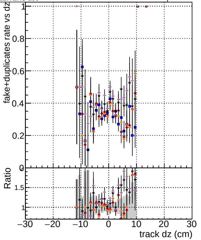
DQM_mkFit_TToriginal DQM_mkFit_TToriginal-106 DQM_mkFit_TTNEWHSMS95_ALLITERS-106 DQM_mkFit_TTNEWHSMS95chi2_ALLITERS-106 DQM_mkFit_TTNEWHSMS95dpdq_ALLITERS-106
