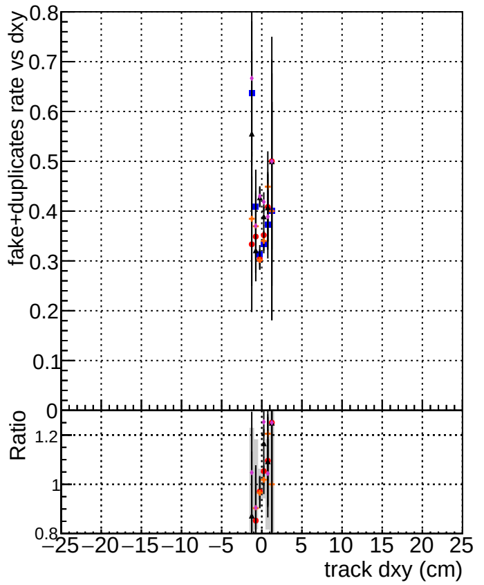
DQM_mkFit_TToriginal DQM_mkFit_TToriginal-106 DQM_mkFit_TTNEWHSMS95_ALLITERS-106 DQM_mkFit_TTNEWHSMS95chi2_ALLITERS-106 DQM_mkFit_TTNEWHSMS95dpdq_ALLITERS-106
