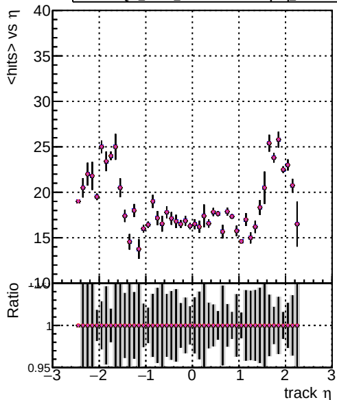
Legend for mean hits vs track \eta : DOM mkFit Toriginal-106 DOM mkFit TNEWHSMS95 ALLITERS-106 DOM mkFit TNEWHSMS95ch2 ALLITERS-106 DOM mkFit TNEWHSMS95dpg ALLITERS-106
