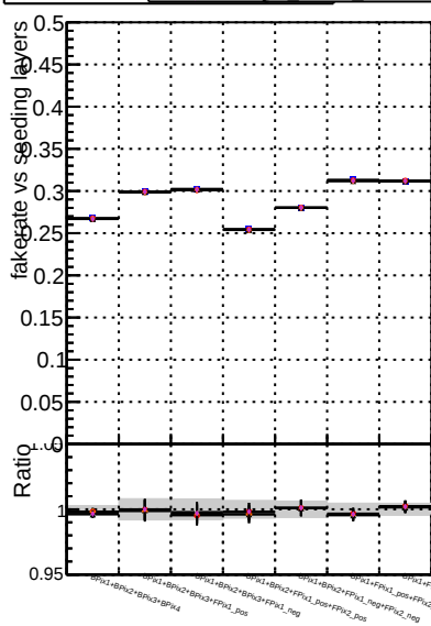
Fake rate vs. Legend: DOM, mkFit, T, Original, TFS, ALLPERS-106, NEWHSM395, NEWHSM395-106, ALLPERS-106
