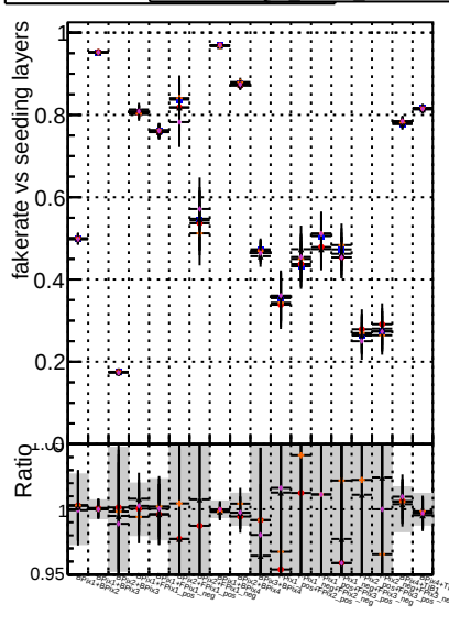
Fake rate vs. DOM mkFit Toriginal vs ALLPERS-106
