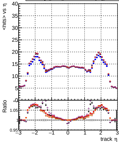
mean hits DOM mkFit Toriginal-106 DOM mkFit TNEWHSM95 ALLITERS-106 DOM mkFit TNEWHSM95ch2 ALLITERS-106 DOM mkFit TNEWHSM95dpdg ALLITERS-106
