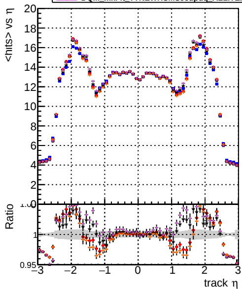
mean hit DOM mkFit Toriginal-106 DOM mkFit TNEWHSMS95 ALLITERS-106 DOM mkFit TNEWHSMS95ch2 ALLITERS-106 DOM mkFit TNEWHSMS95dpdg ALLITERS-106
