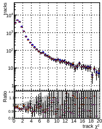
N of reco track vs. \chi^2 for BDM mFit TFit TFit+T NEWFSM ALL LITERS-106 ALL LITERS-106
