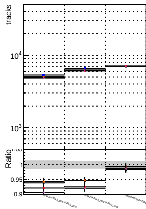
N of reco track vs. \chi^2 for BDM mFit TFit TFit+T NEWFSM ALL LITERS-106 ALL LITERS-106
