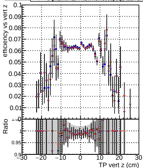
Efficiency vs vert z DOM mkFit Toriginal-106 DOM mkFit TNEWHSMS95 ALLITERS-106 DOM mkFit TNEWHSMS95chi2 ALLITERS-106 DOM mkFit TNEWHSMS95dpdg ALLITERS-106
