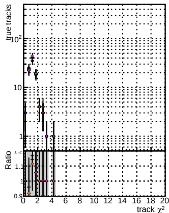
N of reco track vs. \chi^2 for various methods and datasets. Legend: DOM (black), mFit (red), TFit (blue), TFit+106 (green), TFit+106+106 (orange). Datasets: ALL (black), LITERS-106 (red), NEWISM-3000 (blue), LITERS-106 (green).
