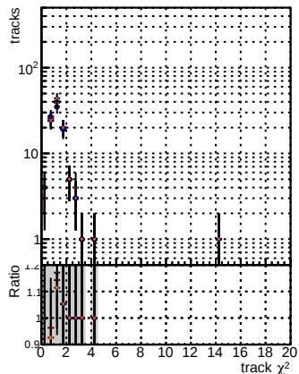
N of reco track vs. \chi^2 for various methods and datasets. Legend: DOM (black), mFit (red), TFit (blue), TFit+106 (green), TFit+106+106 (orange). Datasets: ALL (black), LITERS-106 (red), NEWISM-3000 (blue), LITERS-106 (green).
