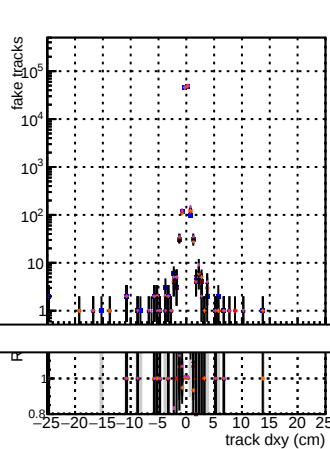
N of associated (recoToSim) loopers tracks vs dxy
