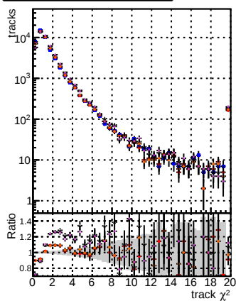
N of reco track vs. \chi^2 for BOM, mFit, TFit, and TFit+TTC
