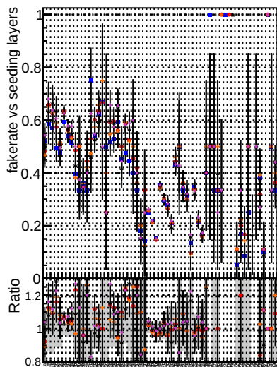
Fake rate vs. DOM mktFit T Original vs ALLPERS-106 DOM mktFit T NEWHSM395800g ALLPERS-106
