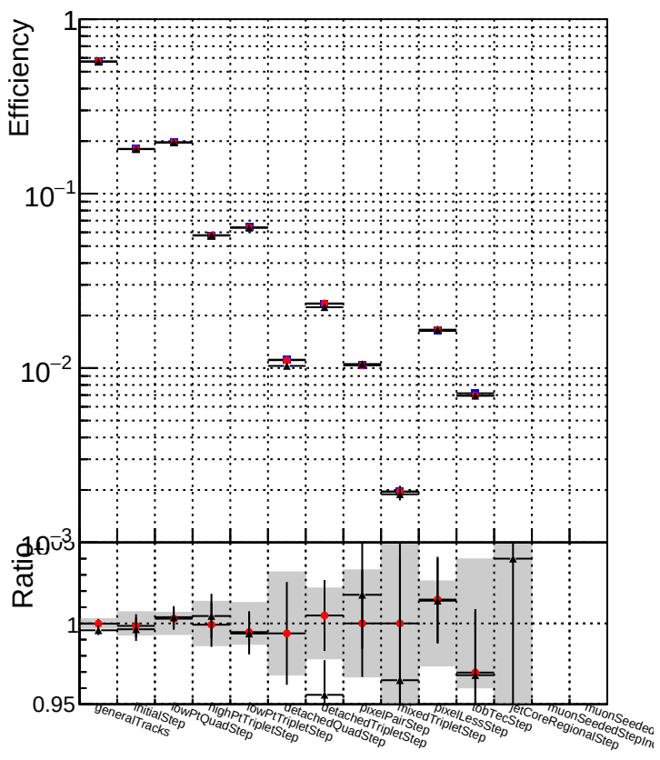
DQM_mkFit_TToriginal DQM_mkFit_TTNEWHWS_ALLITERS DQM_mkFit_TTNEWHSMS_ALLITERS
