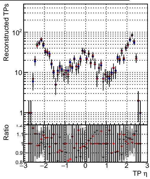
N of simulated tracks vs \eta Legend: DQM_mkFit_TToriginal (blue dots) DQM_mkFit_TTNEWSMS_ALLITERS (red dots) DQM_mkFit_TTNEWSMS_ALLITERS (black dots)
