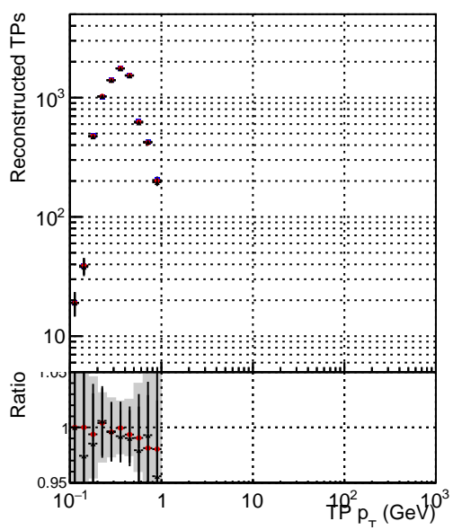
● DQM_mkFit_TToriginal ● DQM_mkFit_TTNEWSMS_ALLITERS ● DQM_mkFit_TTNEWSMS_ALLITERS
