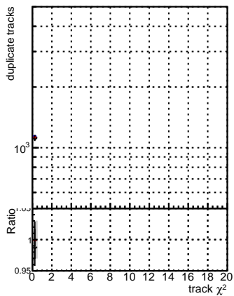
N of associated (recoToSim) loopier tracks vs. \chi^2 for different track selection criteria
