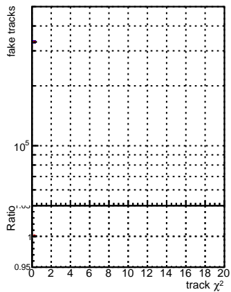
N of fake tracks vs. \chi^2 for different track selection criteria
