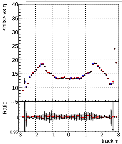
mean hit — DQM_mkFit_TToriginal — DQM_mkFit_TTNEVHS_ALLITERS — DQM_mkFit_TTNEVHSM ALLITERS
