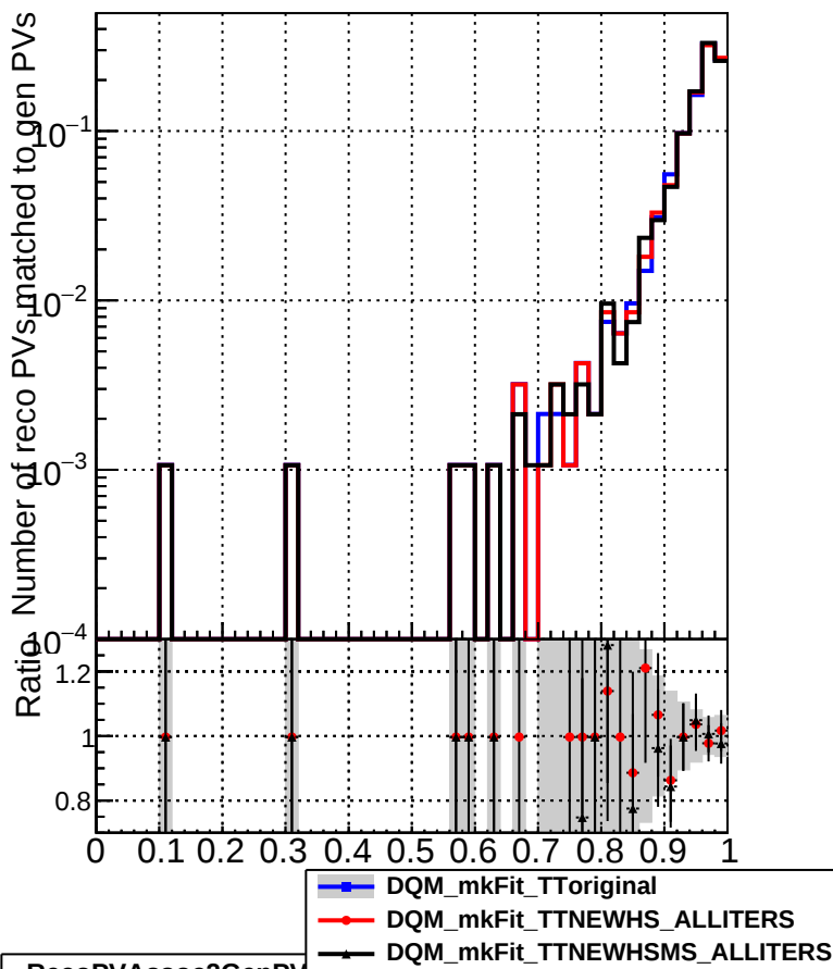
RecoPVAssoc2GenPVmatched_missing
