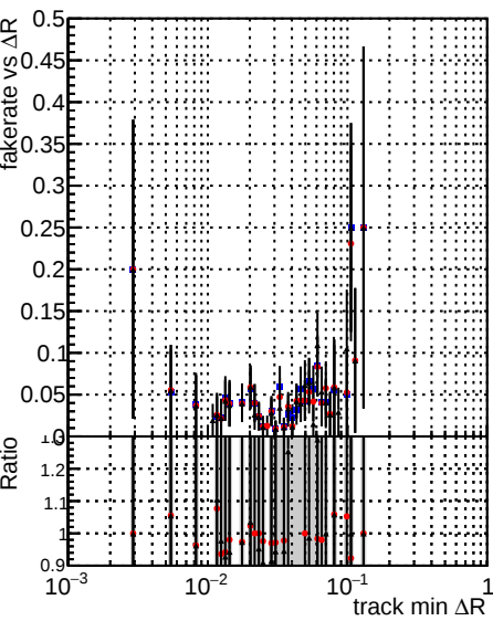
Fake rate vs \Delta R(\text{track}, \text{jet}) Legend: DQM_mkFit_TToriginal (blue dots) DQM_mkFit_TTNEUHS_ALLITERS (red dots) DQM_mkFit_TTNEUHSMS_ALLITERS (black dots)
