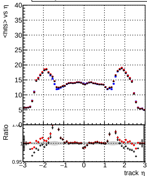
mean hit — DQM_mkFit_TToriginal — DQM_mkFit_TTNEWHS_ALLITERS — DQM_mkFit_TTNEWHSMS_ALLITERS
