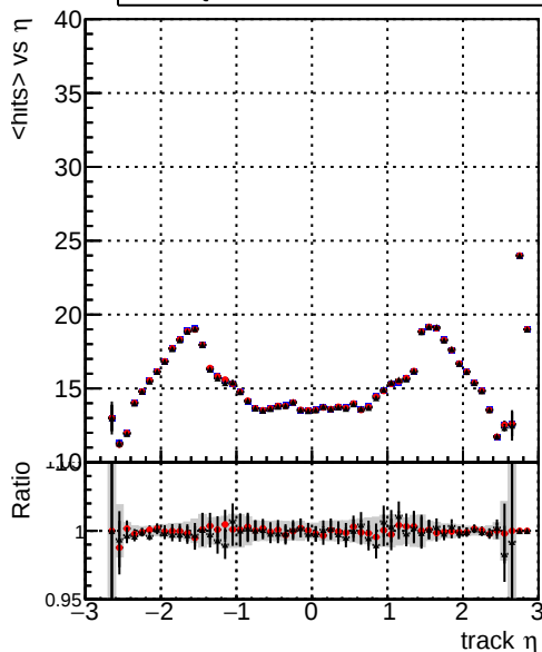
mean hits vs \eta — DQM_mkFit_TToriginal — DQM_mkFit_TTNEWHS_ALLITERS — DQM_mkFit_TTNEWHSMS_ALLITERS
