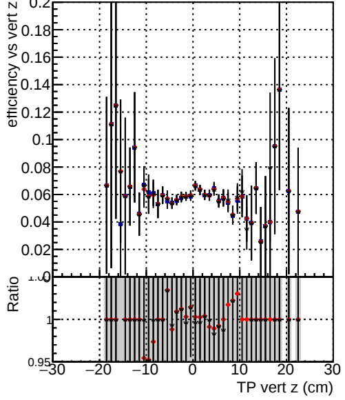
Efficiency vs. TP vert z (cm) Legend: - \bullet DQM_mkFit_TToriginal - \bullet DQM_mkFit_TTNEWHHS_ALLITERS - \bullet DQM_mkFit_TTNEWHSMS_ALLITERS
