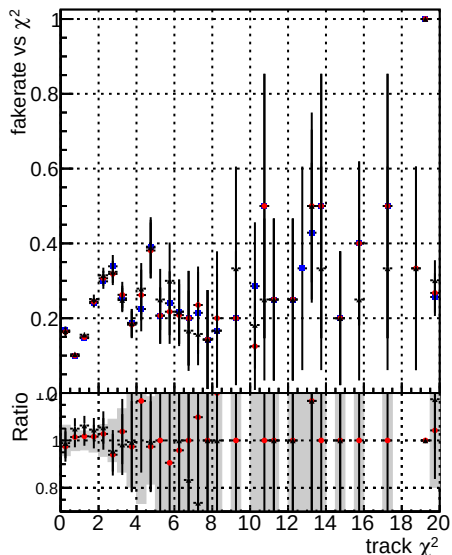
Fake rate vs. DOM mkFit Ttoriginal DOM mkFit Ttoriginal ALLITERS
