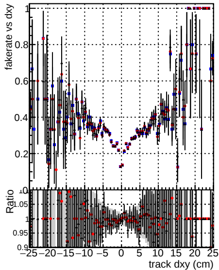
— DOM mkFit TToriginal — DOM mkFit TTNEW — DOM mkFit TTALLITERS
