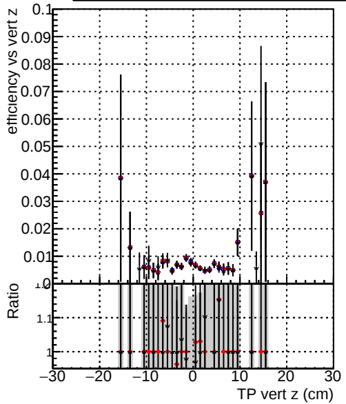
Efficiency vs vert z —●— DQM_mkFit_TToriginal —●— DQM_mkFit_TTNEWHS_ALLITERS —●— DQM_mkFit_TTNEWHSMS_ALLITERS
