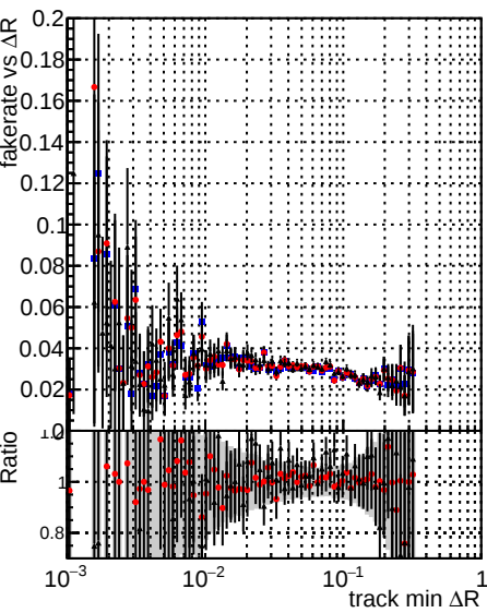
Fake rate vs \Delta R (track, jet) Legend: DQM_mkFit_TToriginal (black line with dots) DQM_mkFit_TTNEUHS_ALLITERS (red line with dots) DQM_mkFit_TTNEUHSMS_ALLITERS (blue line with dots)
