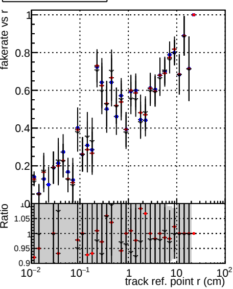
Fake rate vs verpos —●— DQM_mkFit_TToriginal —●— DQM_mkFit_TTNEUHS ALLITERS —●— DQM_mkFit_TTNEUHSMS ALLITERS
