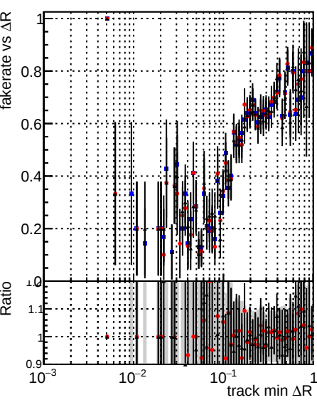
Fake rate vs \Delta R(\text{track, jet}) Legend: DQM_mkFit_TToriginal (blue dots) DQM_mkFit_TTNEWHWS_ALLITERS (red dots) DQM_mkFit_TTNEWHWS_ALLITERS (black dots)
