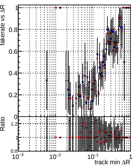
Fake rate vs \Delta R (track, jet) DQM_mkFit_TToriginal DQM_mkFit_TTNEUHS_ALLITERS DQM_mkFit_TTNEUHSMS_ALLITERS
