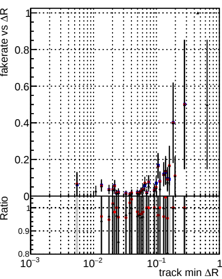
Fake rate vs \Delta R (track, jet) DQM_mkFit_TToriginal DQM_mkFit_TTNEWHS_ALLITERS DQM_mkFit_TTNEWHS_ALLITERS
