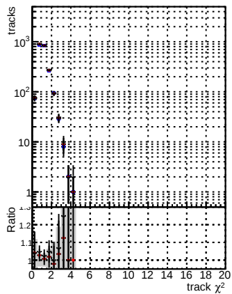
N of reco track vs. \chi^2 for DQM mFit (blue), DQM mFit (red), and DQM mFit (green) for ALL ALTERS
