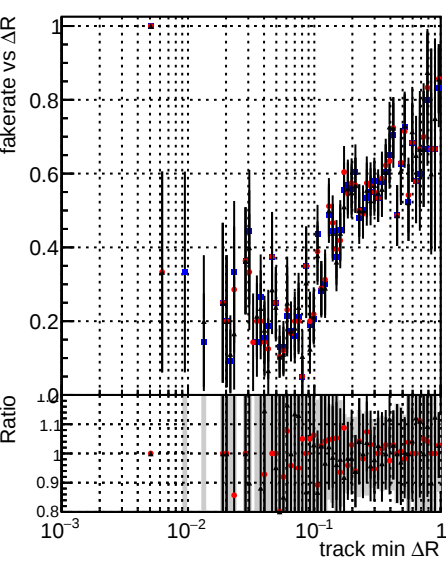
Fake rate vs \Delta R(\text{track, jet}) Legend: DQM_mkFit_TToriginal (blue dots) DQM_mkFit_TTNEWHS_ALLITERS (red dots) DQM_mkFit_TTNEWHSMS_ALLITERS (black dots)
