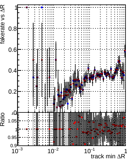
Fake rate vs \Delta R(\text{track, jet}) Legend: DQM_mkFit_TToriginal (blue dots) DQM_mkFit_TTNEWHS_ALLITERS (red dots) DQM_mkFit_TTNEWHSMS_ALLITERS (black crosses)
