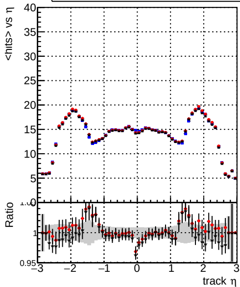
mean hit — DQM_mkFit_TToriginal — DQM_mkFit_TTNEUHS_ALLITERS — DQM_mkFit_TTNEUHSMS_ALLITERS
