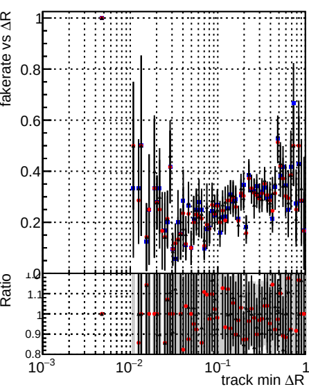
Fake rate vs \Delta R (track, jet) Legend: DQM mkFit TToriginal (blue circles) DQM mkFit TTNEWHS ALLITERS (red circles) DQM mkFit TTNEWHS ALLITERS (black circles)
