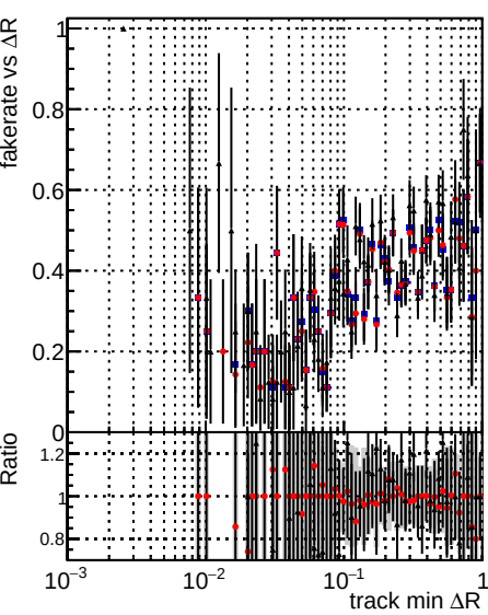
Fake rate vs \Delta R(\text{track, jet}) DQM_mkFit_TToriginal DQM_mkFit_TTNEUHS_ALLITERS DQM_mkFit_TTNEUHS_ALLITERS
