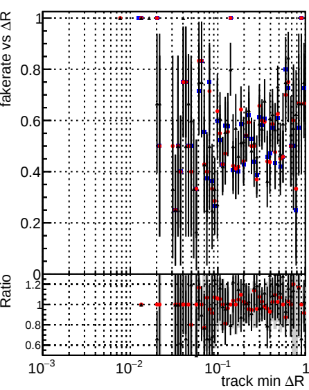
Fake rate vs \Delta R(\text{track, jet}) Legend: DQM_mkFit_TToriginal DQM_mkFit_TTNEWHS_ALLITERS DQM_mkFit_TTNEWHSMS_ALLITERS
