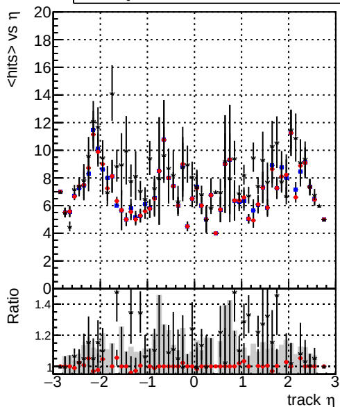
mean hit — DQM_mkFit_TToriginal — DQM_mkFit_TTNEWHWS_ALLITERS — DQM_mkFit_TTNEWHWSMS_ALLITERS
