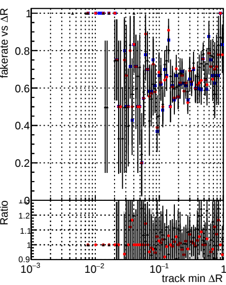
Fake rate vs \Delta R(\text{track, jet}) Legend: DQM_mkFit_TToriginal (black line with dots) DQM_mkFit_TTNEWHWS_ALLITERS (red line with dots) DQM_mkFit_TTNEWHWS_ALLITERS (blue line with dots)
